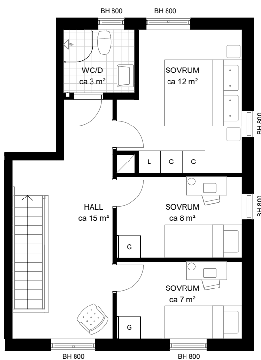
PLAN 2
