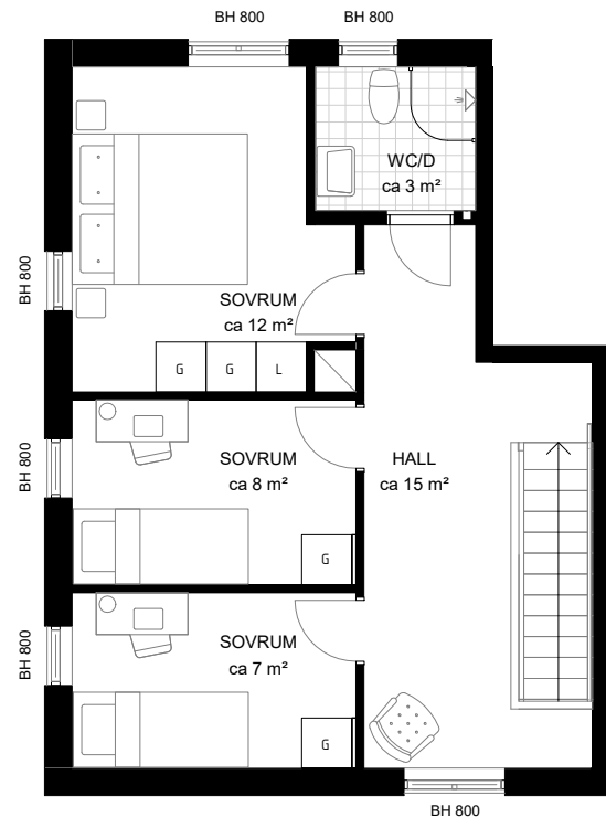
PLAN 2
